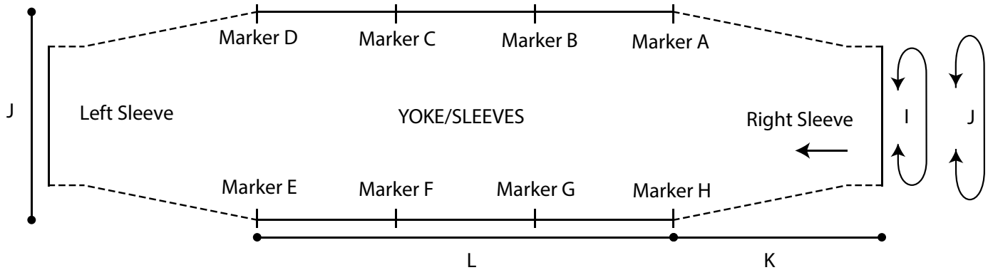
DIAGRAM FOR SIZES 27" / 68.5 cm, 30" / 76 cm, and 33" / 84 cm
